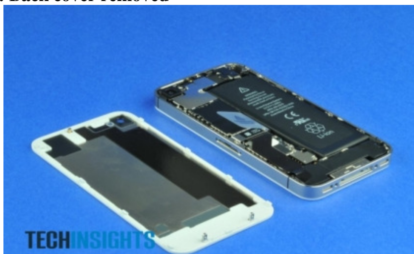
The back cover of the iPhone 4S removed reveals the main board and the battery.
